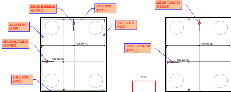
CORE 3 - BOTTOM REINFORCEMENT PLAN
