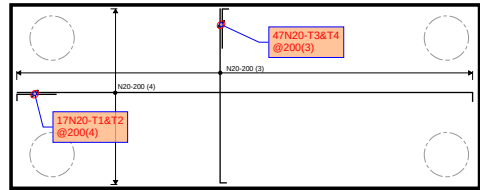
STAIR 1 - TOP REINFORCEMENT PLAN
