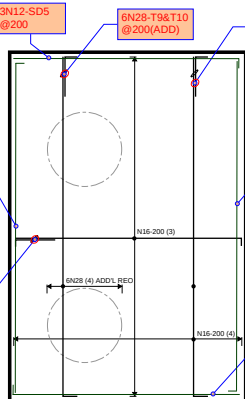
PC3 - TOP REINFORCEMENT PLAN
