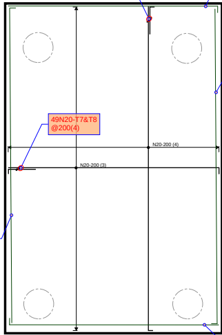
CORE 2 - TOP REINFORCEMENT PLAN
